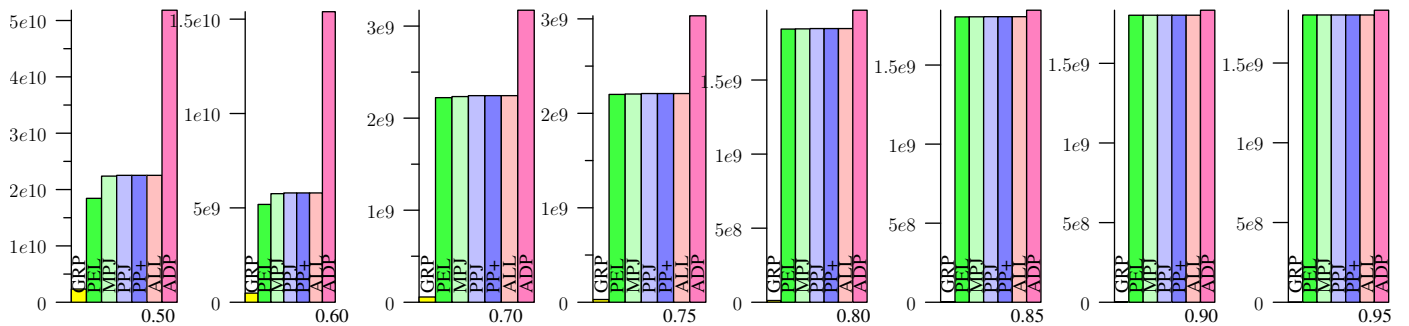
Figure 66: KOSARAK, no deduplication, Jaccard
