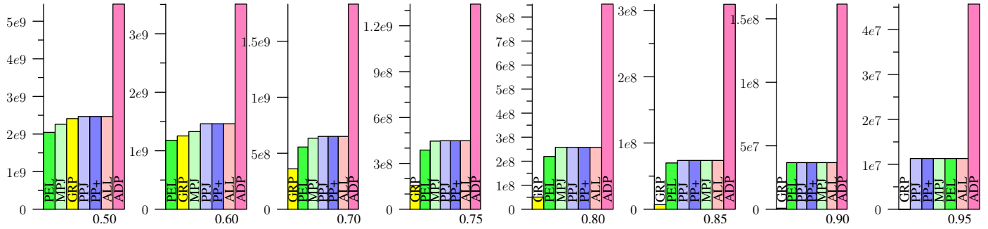
Figure 71: UNIFORM, Jaccard
