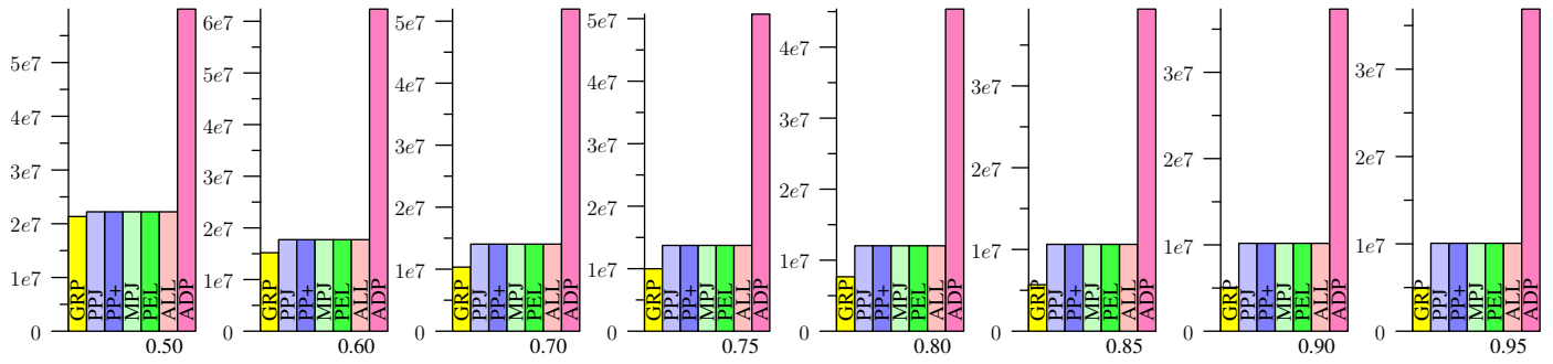
Figure 47: AOL, Jaccard
