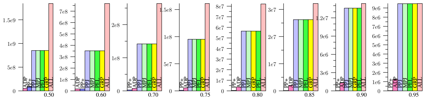
Figure 74: BMS-POS, Jaccard
