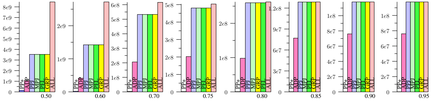
Figure 73: AOL, Jaccard
