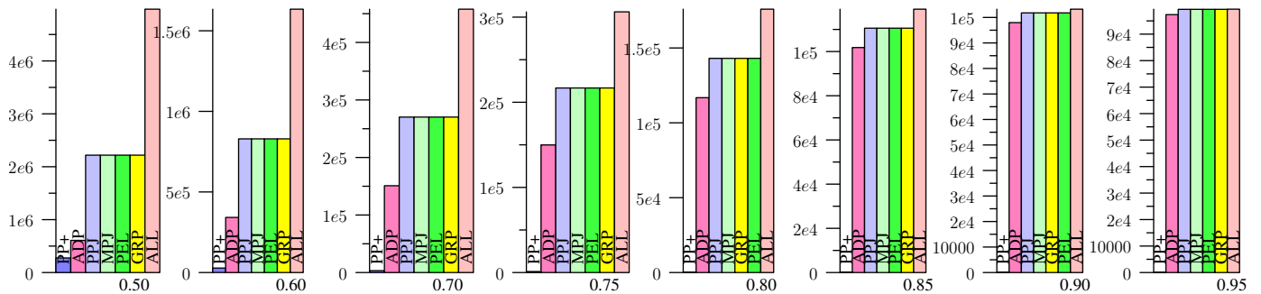
Figure 83: SPOT, Jaccard
