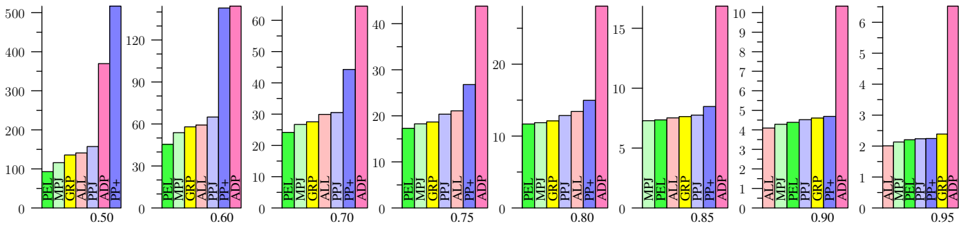
Figure 43: ORKUT, Jaccard
