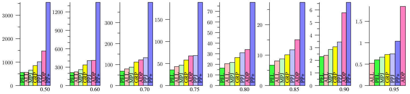
Figure 42: NETFLIX, Jaccard
