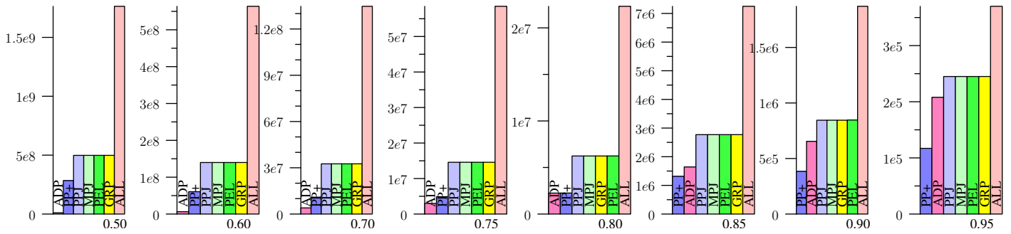
Figure 76: ENRON, Jaccard
