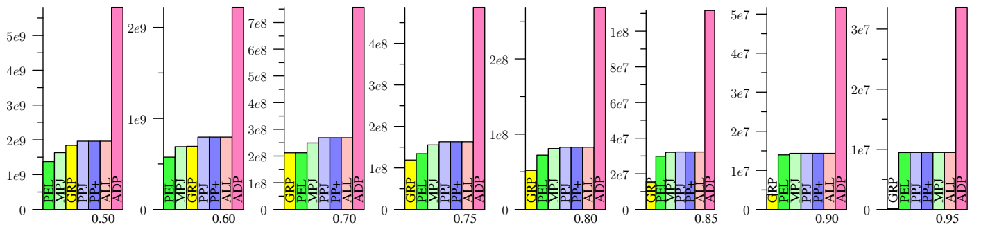
Figure 61: BMS-POS, Jaccard
