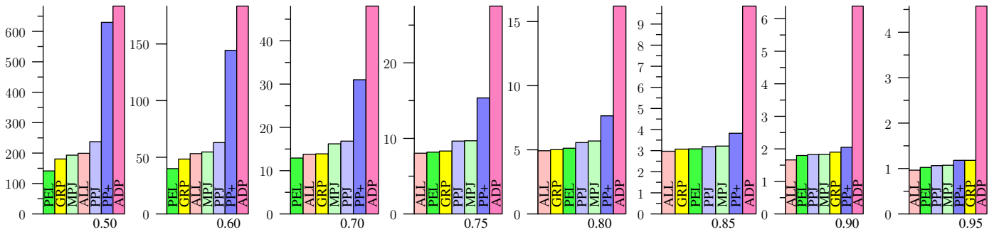
Figure 41: LIVEJ, Jaccard
