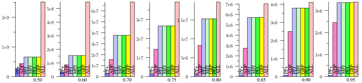
Figure 78: KOSARAK, Jaccard
