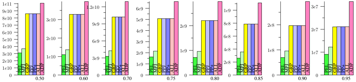
Figure 68: NETFLIX, Jaccard
