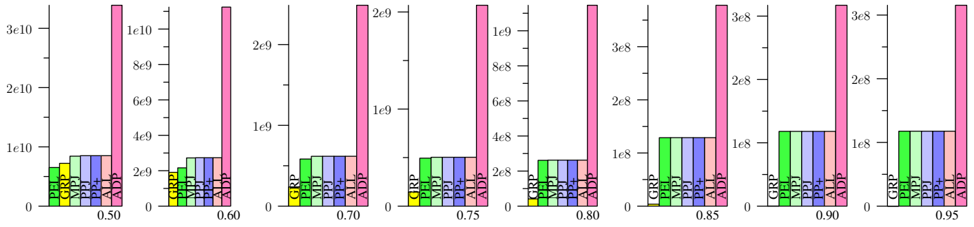
Figure 60: AOL, Jaccard
