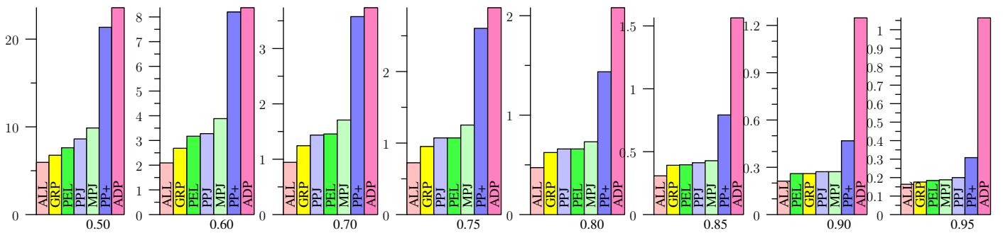
Figure 38: FLICKR, Jaccard
