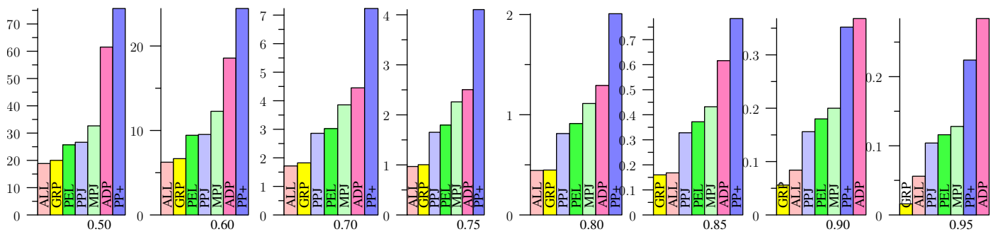
Figure 35: BMS-POS, Jaccard
