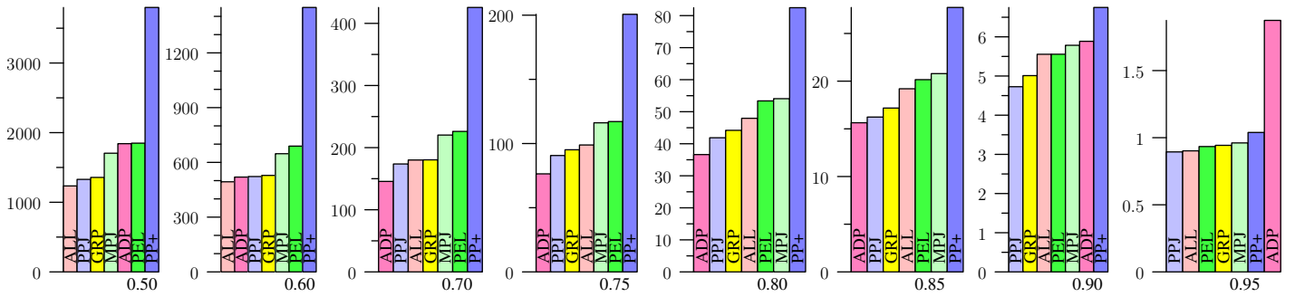
Figure 29: NETFLIX, Jaccard
