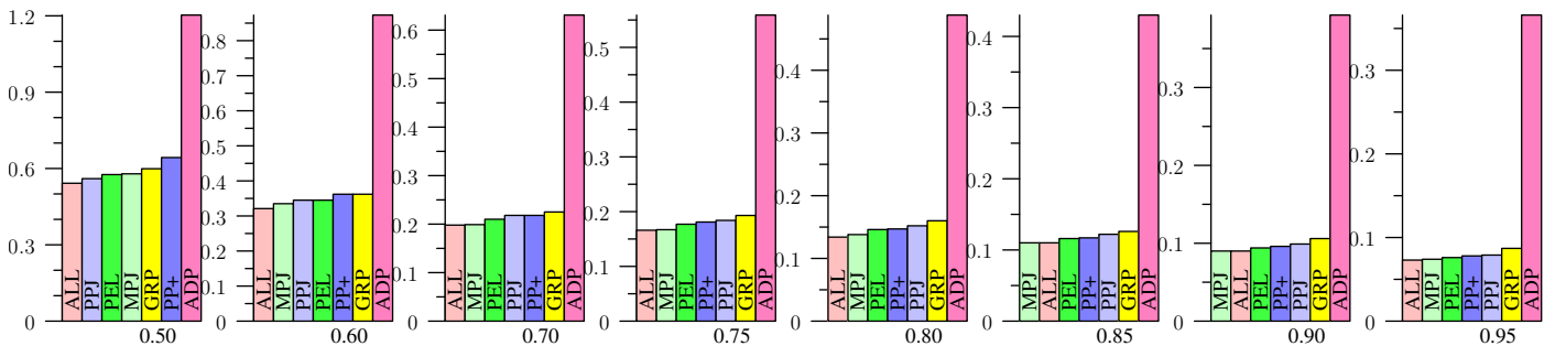
Figure 31: SPOT, Jaccard
