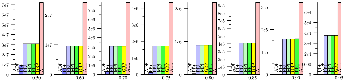
Figure 85: ZIPF, Jaccard
