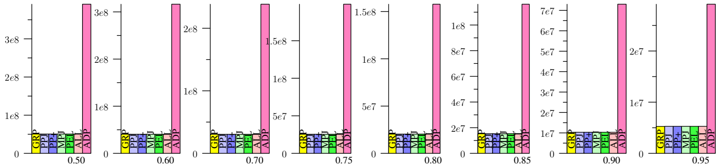
Figure 55: NETFLIX, Jaccard
