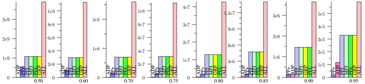
Figure 82: ORKUT, Jaccard
