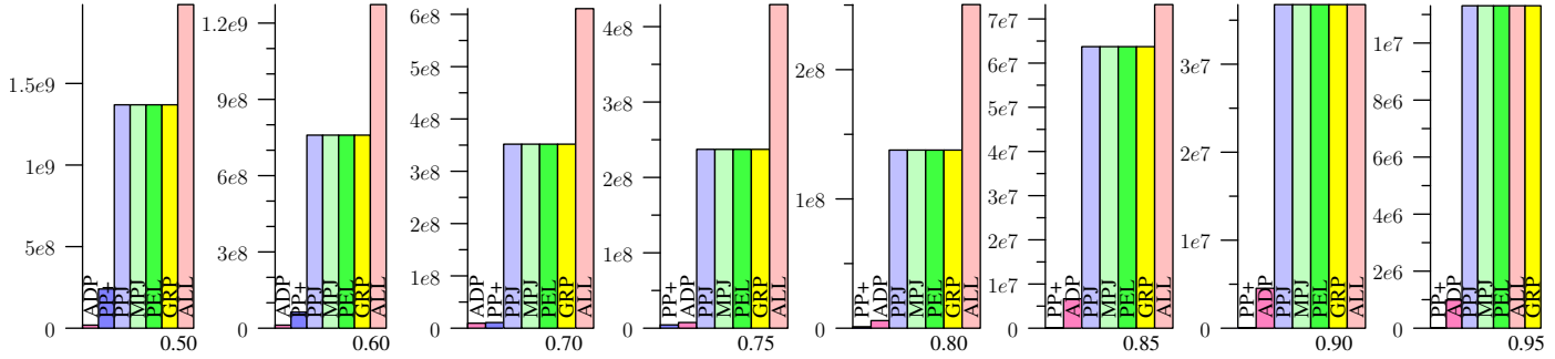
Figure 84: UNIFORM, Jaccard
