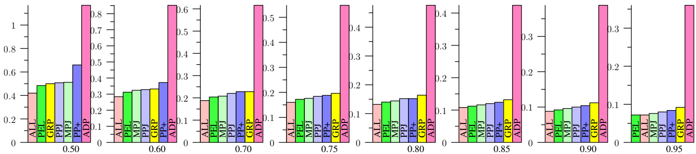
Figure 44: SPOT, Jaccard
