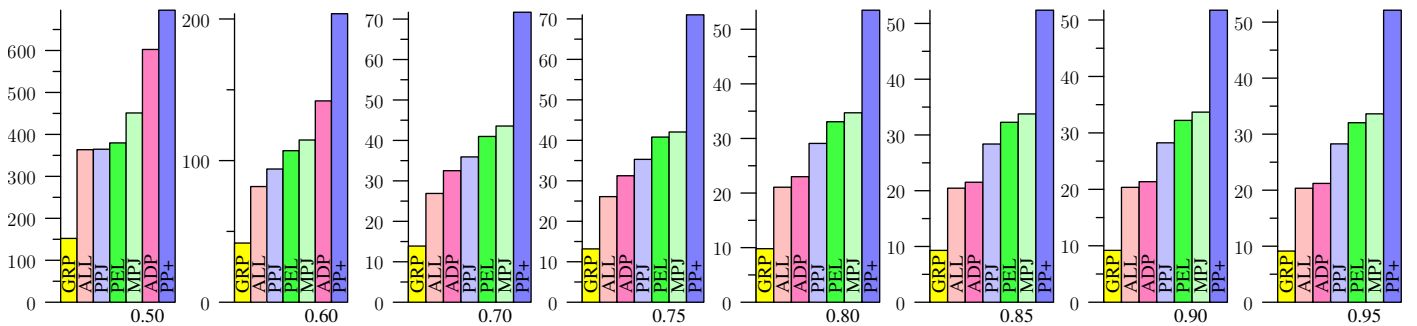
Figure 27: KOSARAK, no deduplication, Jaccard
