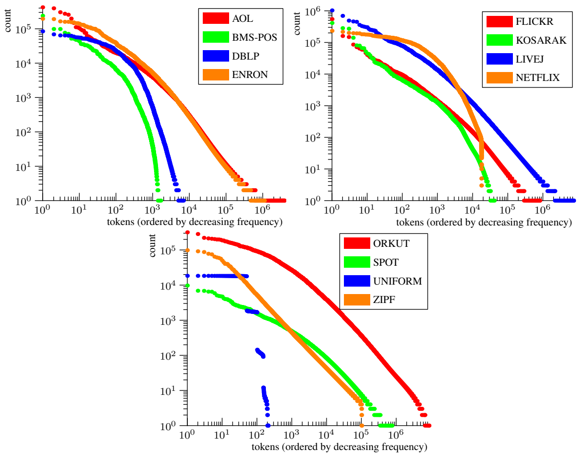
Figure 86: Token frequency distributions
