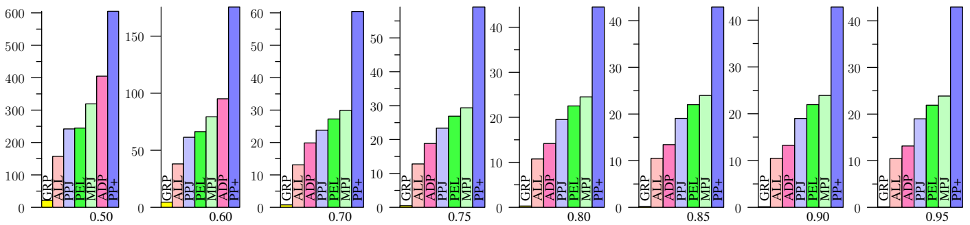
Figure 40: KOSARAK, no deduplication, Jaccard
