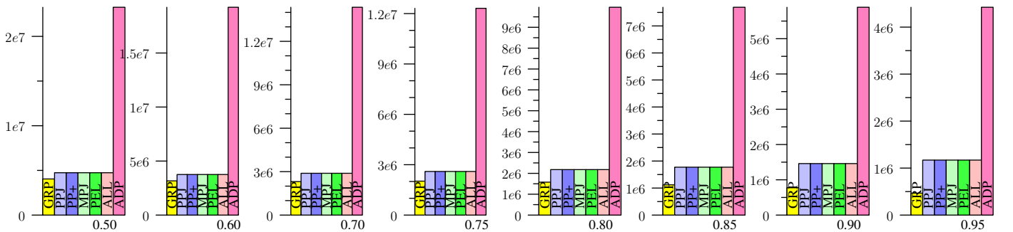
Figure 53: KOSARAK, no deduplication, Jaccard
