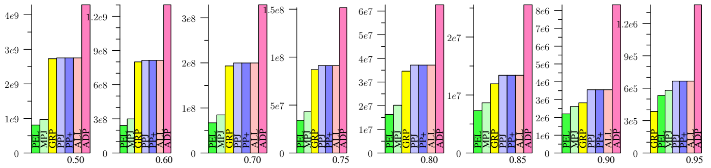
Figure 63: ENRON, Jaccard
