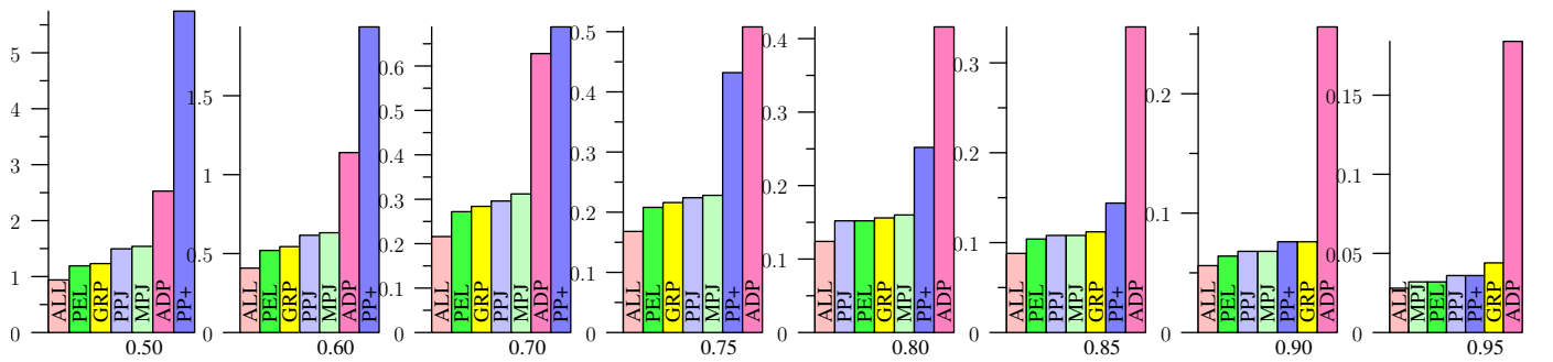
Figure 46: ZIPF, Jaccard
