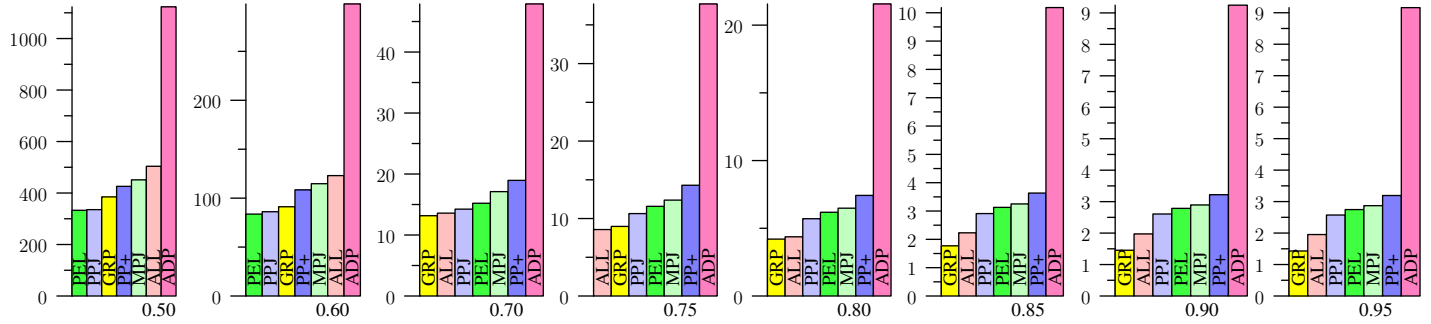
Figure 21: AOL, Jaccard
