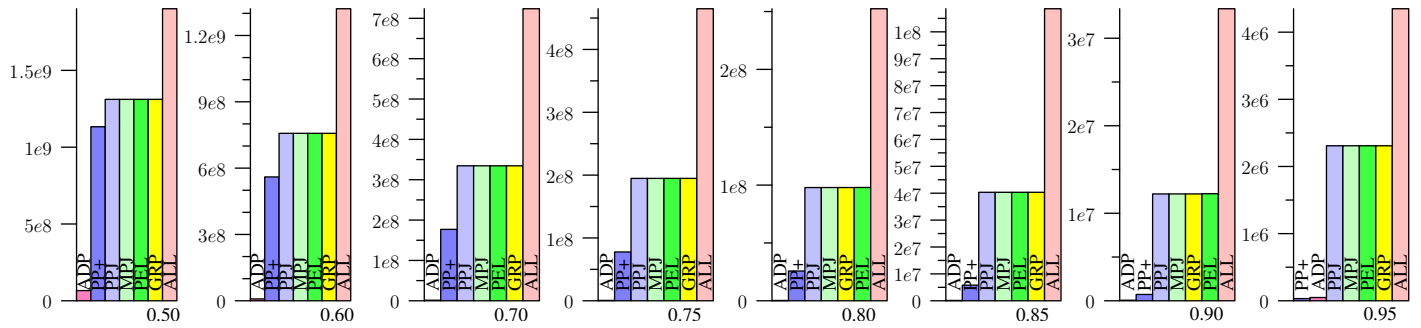
Figure 75: DBLP, Jaccard
