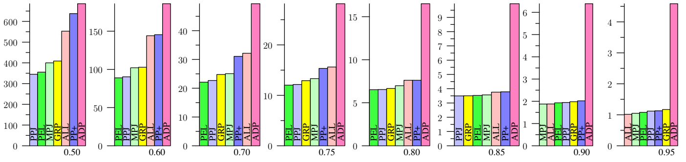
Figure 28: LIVEJ, Jaccard
