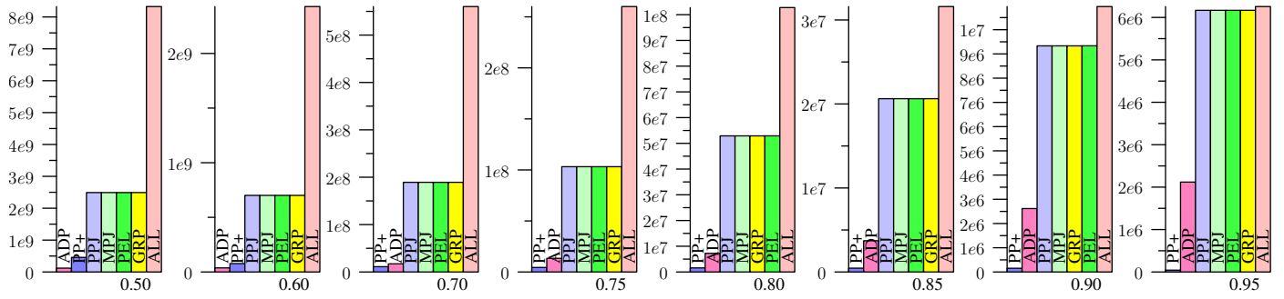
Figure 80: LIVEJ, Jaccard
