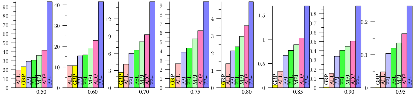
Figure 45: UNIFORM, Jaccard
