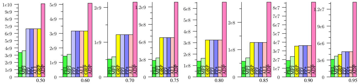
Figure 62: DBLP, Jaccard
