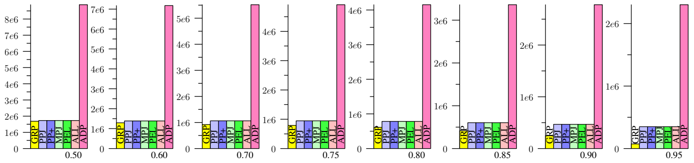
Figure 48: BMS-POS, Jaccard
