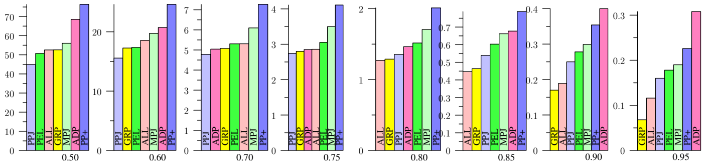
Figure 22: BMS-POS, Jaccard
