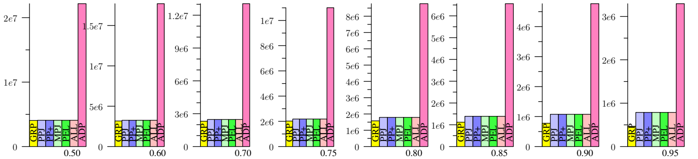
Figure 52: KOSARAK, Jaccard
