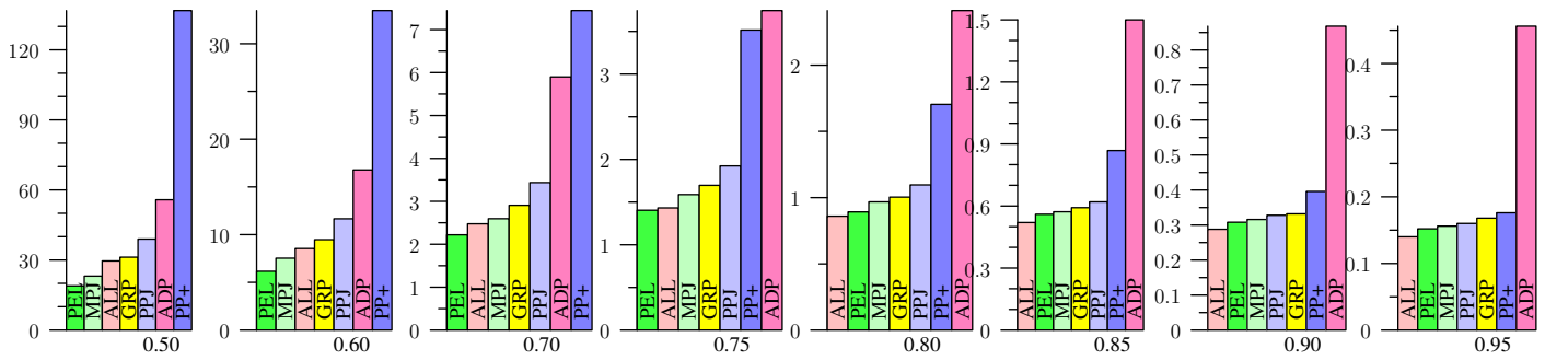
Figure 37: ENRON, Jaccard
