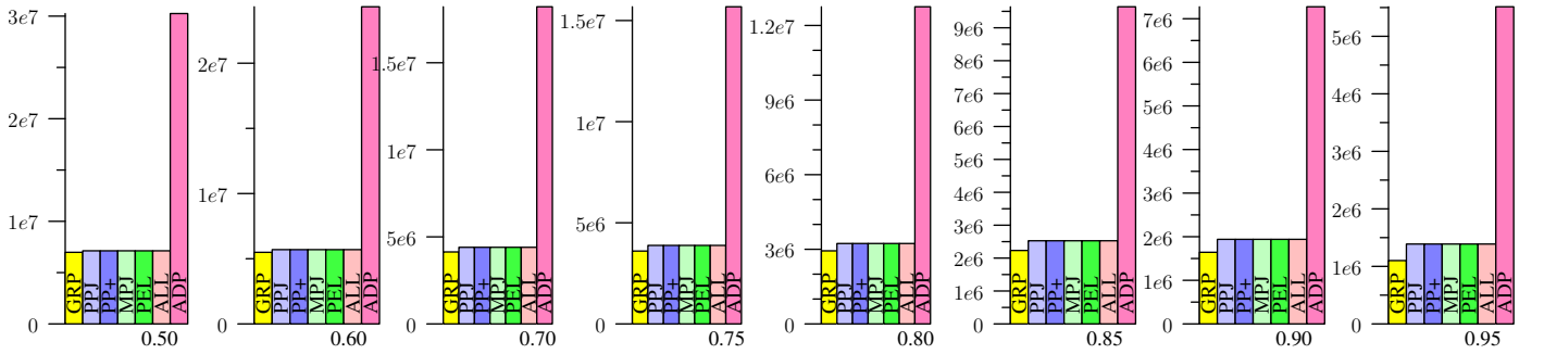
Figure 51: FLICKR, Jaccard
