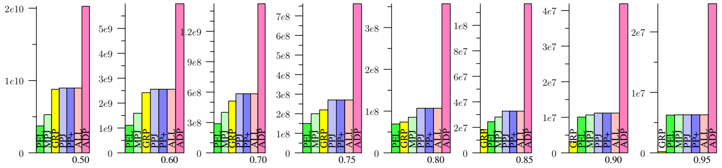
Figure 67: LIVEJ, Jaccard
