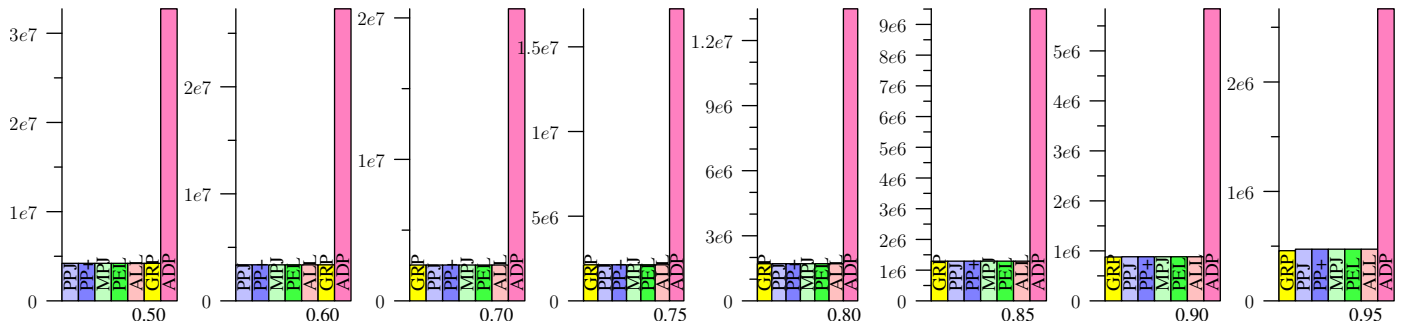
Figure 49: DBLP, Jaccard
