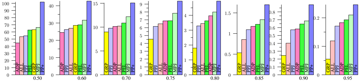
Figure 32: UNIFORM, Jaccard
