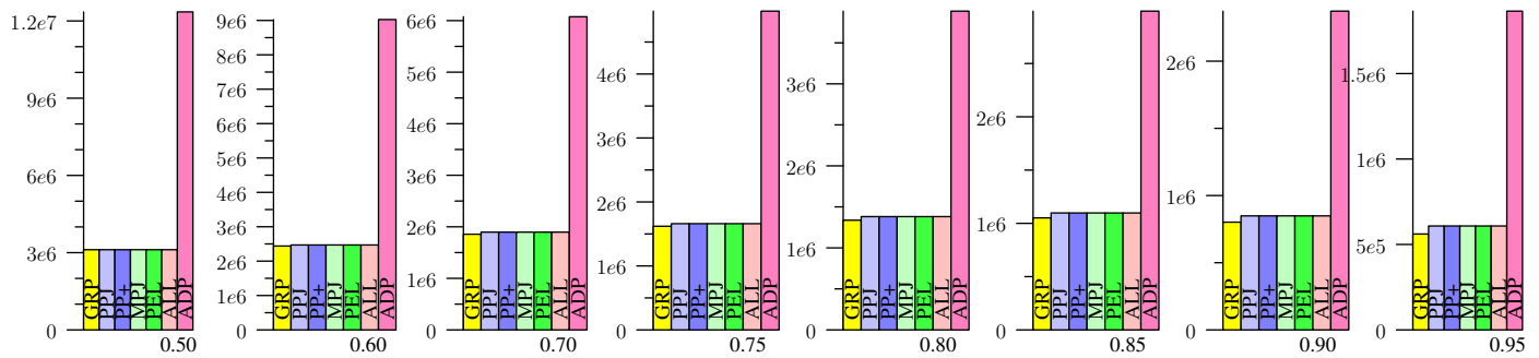
Figure 57: SPOT, Jaccard
