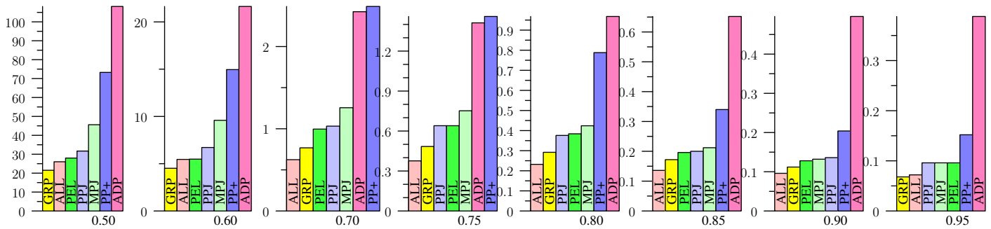
Figure 39: KOSARAK, Jaccard
