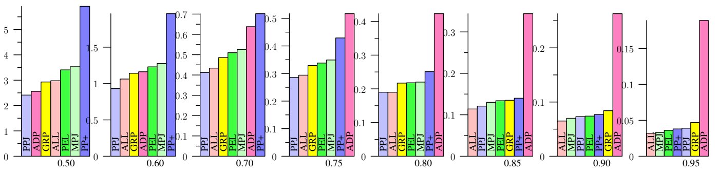
Figure 33: ZIPF, Jaccard
