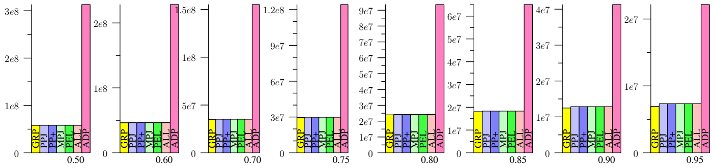
Figure 54: LIVEJ, Jaccard
