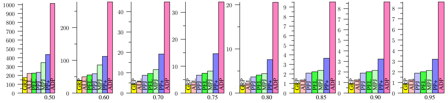
Figure 34: AOL, Jaccard
