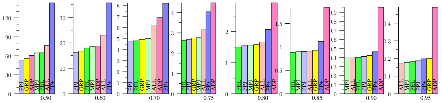
Figure 24: ENRON, Jaccard
