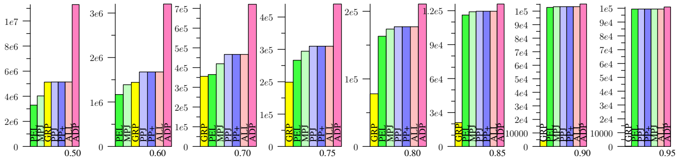
Figure 70: SPOT, Jaccard
