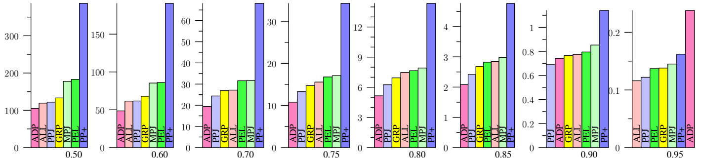
Figure 23: DBLP, Jaccard
