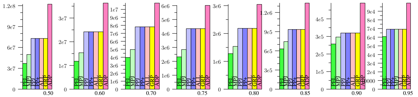
Figure 72: ZIPF, Jaccard
