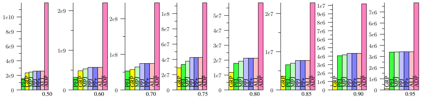
Figure 65: KOSARAK, Jaccard
