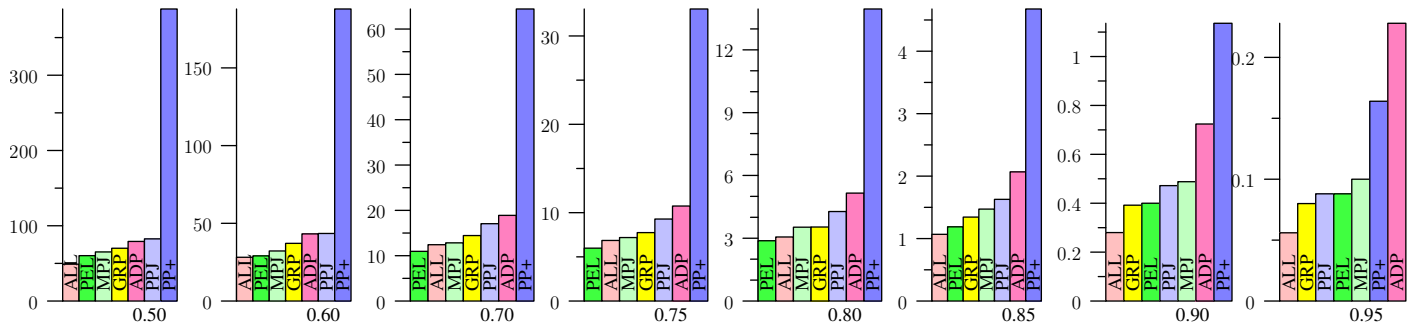
Figure 36: DBLP, Jaccard
