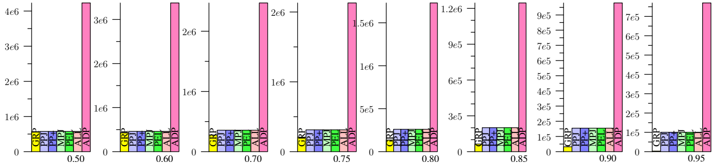
Figure 58: UNIFORM, Jaccard
