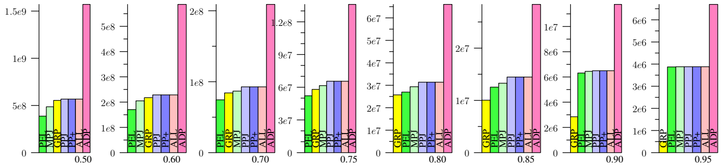
Figure 64: FLICKR, Jaccard
