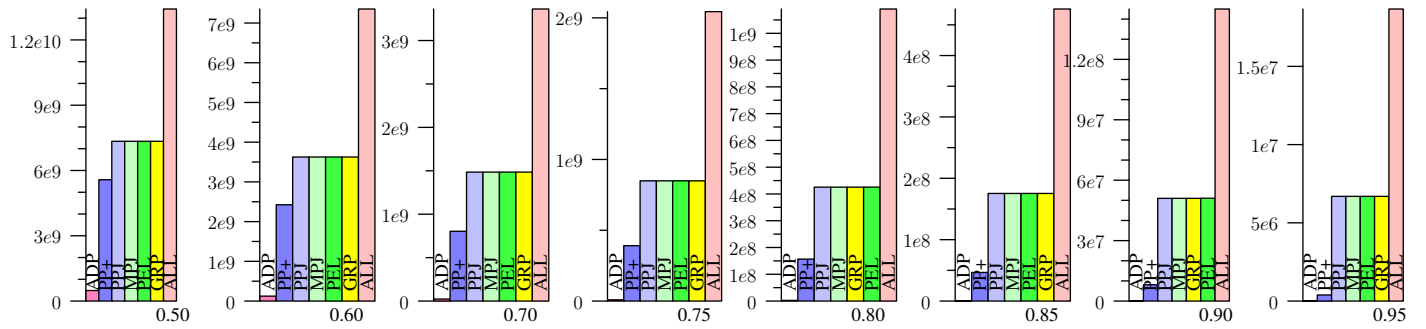
Figure 81: NETFLIX, Jaccard
