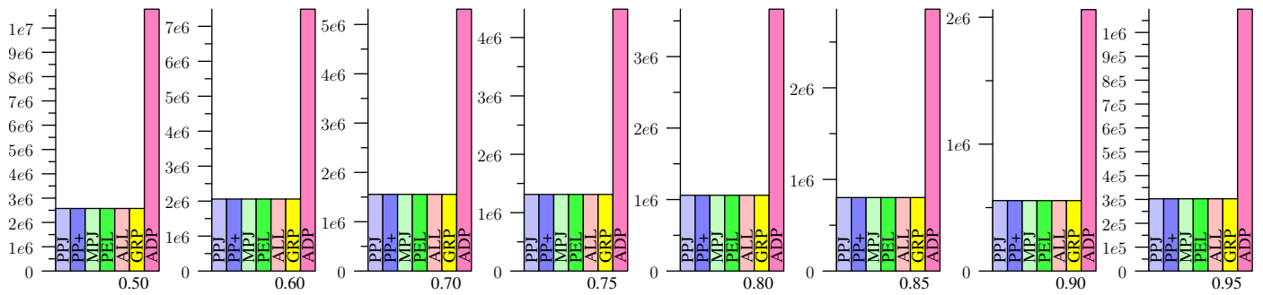
Figure 59: ZIPF, Jaccard
