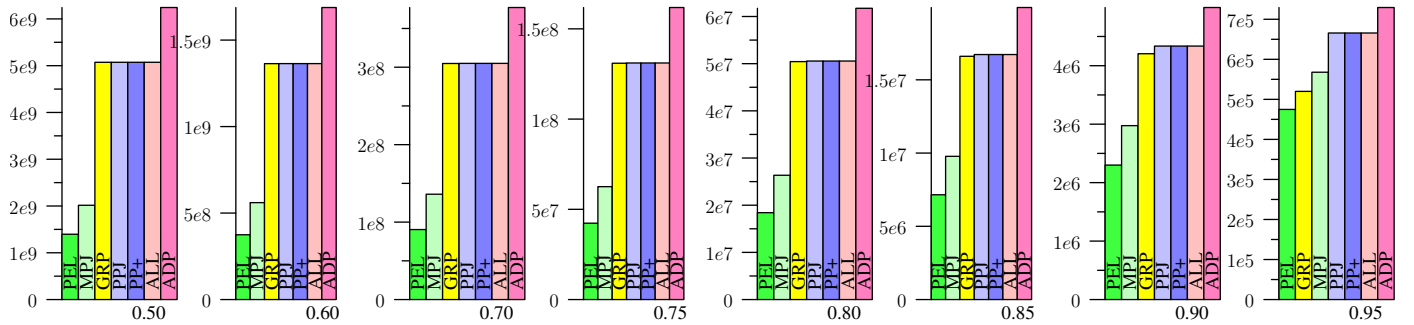
Figure 69: ORKUT, Jaccard
