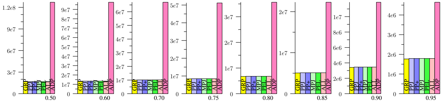
Figure 50: ENRON, Jaccard
