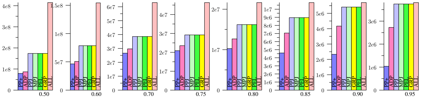
Figure 77: FLICKR, Jaccard
