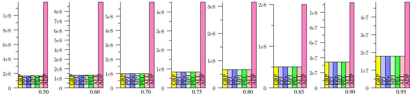
Figure 56: ORKUT, Jaccard
