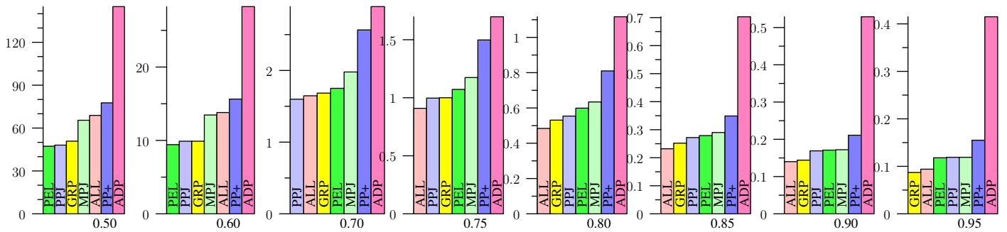
Figure 26: KOSARAK, Jaccard
