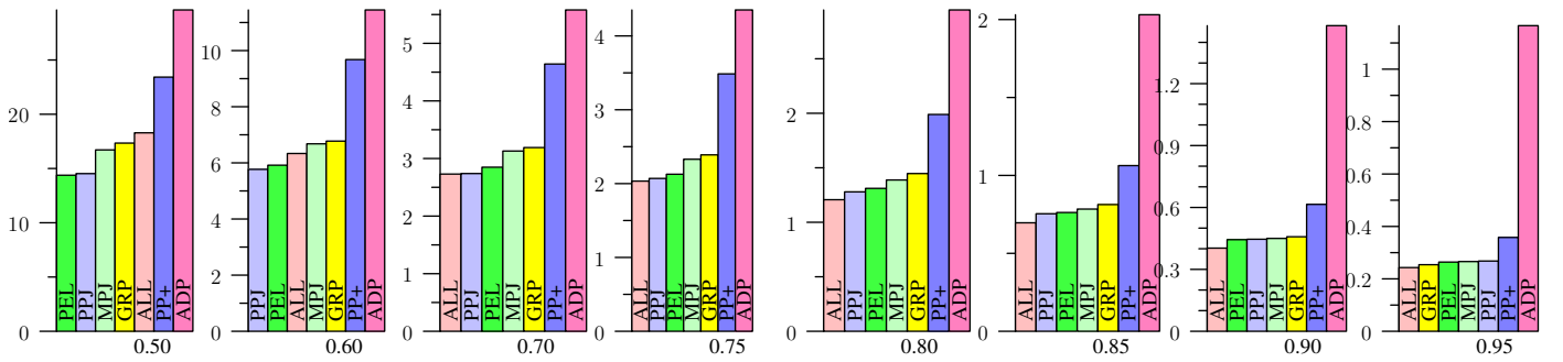
Figure 25: FLICKR, Jaccard
