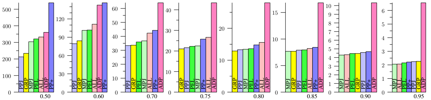
Figure 30: ORKUT, Jaccard
